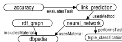
FIGURE 1: A small KG containing research concepts relevant to the Semantic Web domain.
