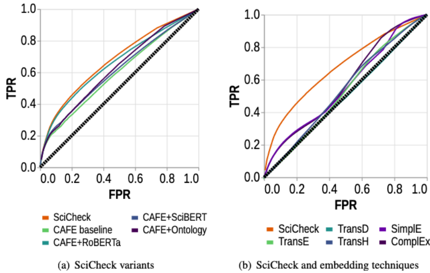
FIGURE 2: ROC curves of the different methods on AIKG-1M.
