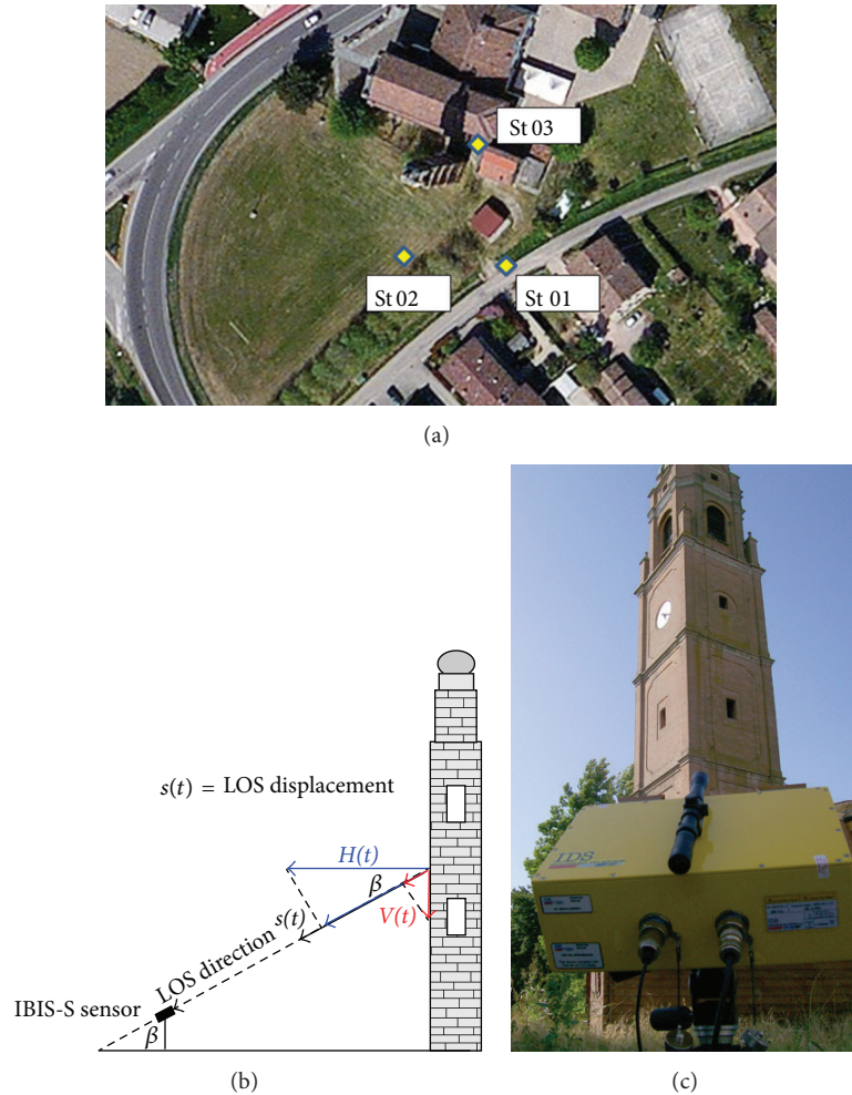
FIGURE 2: (a) Installation of the IBIS-S system in several acquisition stations placed at 25 m (St 01) and 23 m (St 02) from the base of the tower with LOS angle of 30^\circ (central beam) and at 8 m (St 03) with LOS angle of 70^\circ (central beam). (b) Radar line of sight displacement and true displacement vector. (c) Image of the IBIS-S system used during the experiments.
