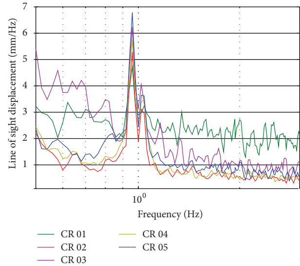
FIGURE 4: Displacement spectra calculated by using the entire 10-minute record, for five different radar-bins with variable SNR achieved from data acquisition with configuration 1.
