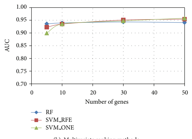
(b) Multivariate ranking methods
