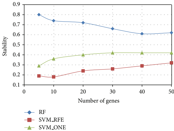
(b) Multivariate ranking methods
