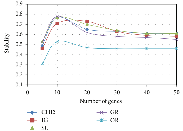
(a) Univariate ranking methods
