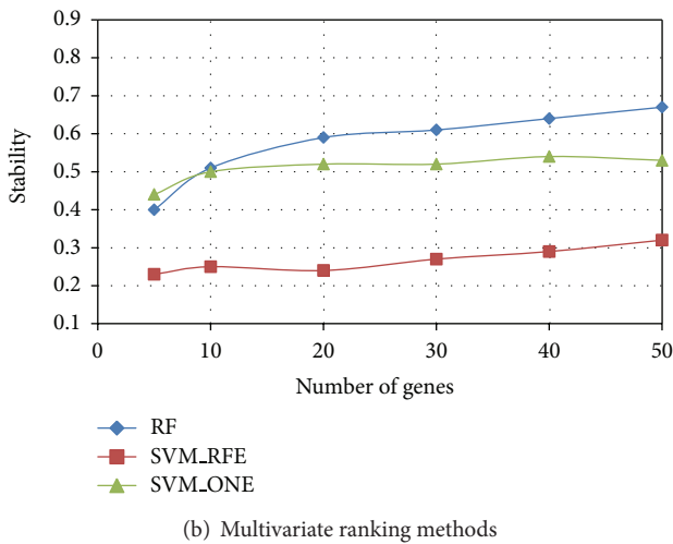
FIGURE 5: Prostate dataset: stability versus number of genes.
