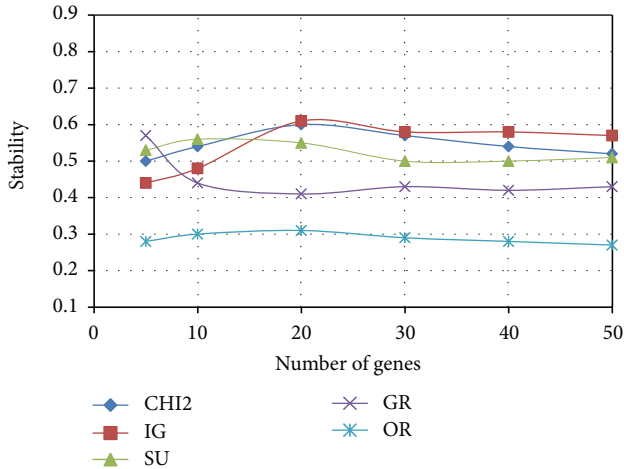
(a) Univariate ranking methods
