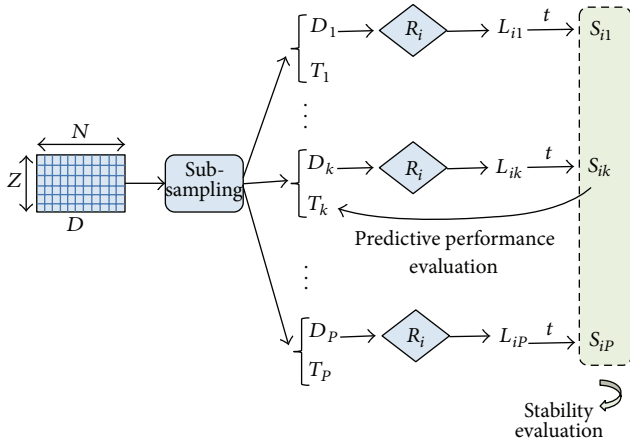
FIGURE 2: Joint evaluation of stability and predictive performance.
