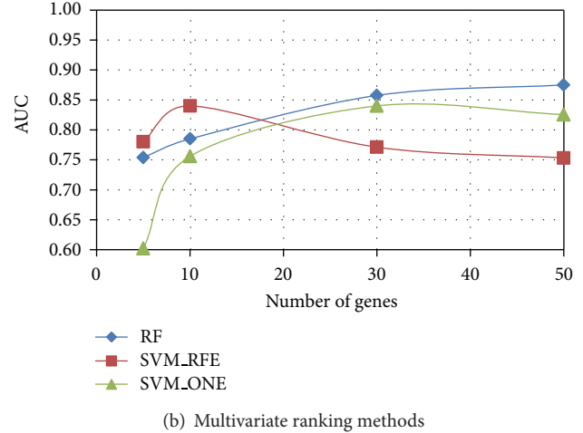
FIGURE 6: Colon dataset: AUC versus number of genes.
