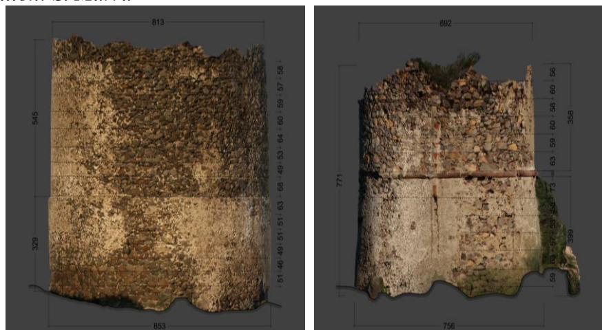
Figure 5. Foghe and Iscra Ruia Tower. Orthogonal Perspective View Highlighting the Dimensional Relations and the Size of the ‘Cantieri’. Graphic Realization: S. Murreu
