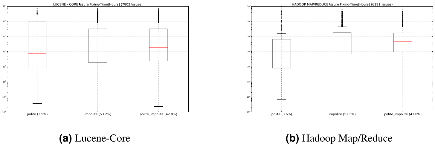
Figure 6 Box-plot of the fixing-time expressed in Hours for single projects. The number in parentheses next to polite/impolite indicates the percentage of impolite and polite issues.
