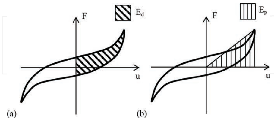
Figure 6. Pinched hysteresis loop (third cycle): (a) dissipated energy for a half cycle; (b) potential energy of the equivalent oscillator for a half cycle.
