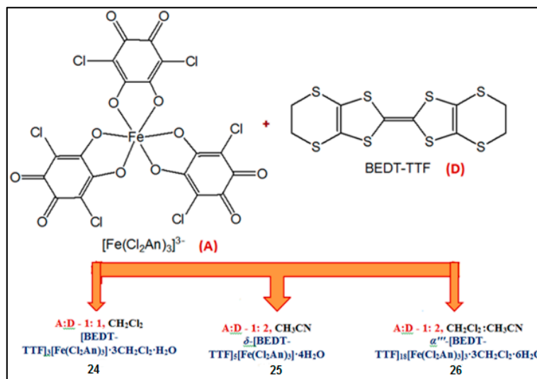
Scheme 8. Molecular structures for the complex anion [\text{Fe}(\text{Cl}_2\text{An})_3]^{3-} and the bis(ethylenedithio)tetrathiafulvalene (BEDT-TTF) organic donor, and experimental conditions used for obtaining 24–26 compounds.
