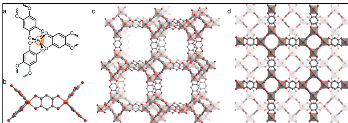
Figure 30. (a) Molecular structure of a single Fe III center in (\text{NBu}_4)_2\text{Fe}^{\text{III}}_2(\text{H}_2\text{An})_3 , showing that two radical ( \text{H}_2\text{An}^{3\bullet} ) bridging ligands and one diamagnetic ( \text{H}_2\text{An}^{2-} ) bridging ligand are coordinated to each metal site; (b) A portion of its crystal structure, showing the local environment of two \text{H}_2\text{An}^{3\bullet} -bridged Fe III centers; (c) A larger portion of the crystal structure, showing one of the two interpenetrated (10,3)-a nets that together generate the porous three-dimensional structure; (d) The two interpenetrated (10,3)-a lattices of opposing chiralities. Charge-balancing \text{NBu}_4^+ cations are not depicted for clarity. Reprinted with permission from Reference [185]. Copyright 2015 American Chemical Society.
