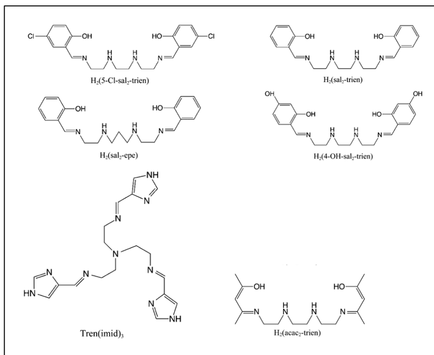
Chart 4a. Ligands of Fe(III) and Fe(II) complexes.
