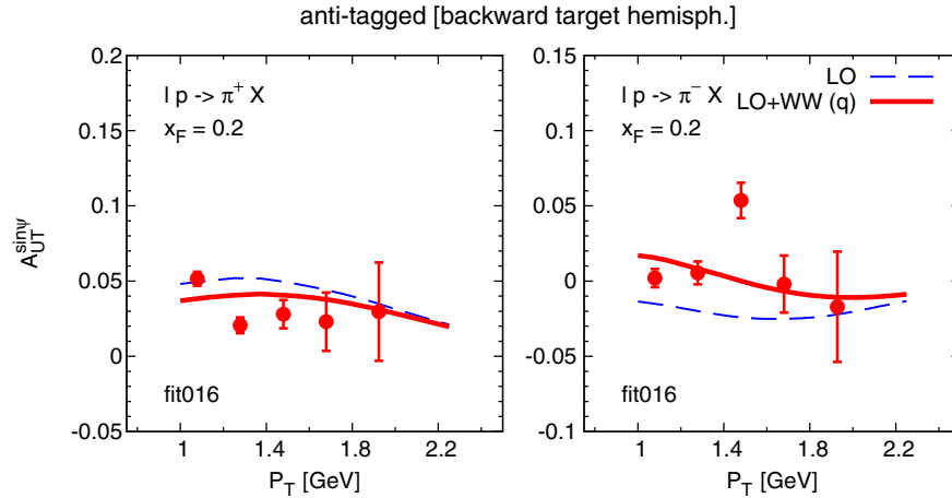
FIG. 13. Theoretical estimates of the Siverson contribution to A_{UT}^{\sin\psi} vs P_T at \sqrt{s} \approx 7.25 GeV and x_F = 0.2 for inclusive \pi^+ (left panel) and \pi^- (right panel) production in \ell p^\uparrow \rightarrow \pi X processes, compared with the antitagged HERMES data [27] and adopting the quark Siverson functions of Ref. [57]. Curves have the following meaning: blue dashed lines for the LO and red solid lines for the LO + WW contributions.
