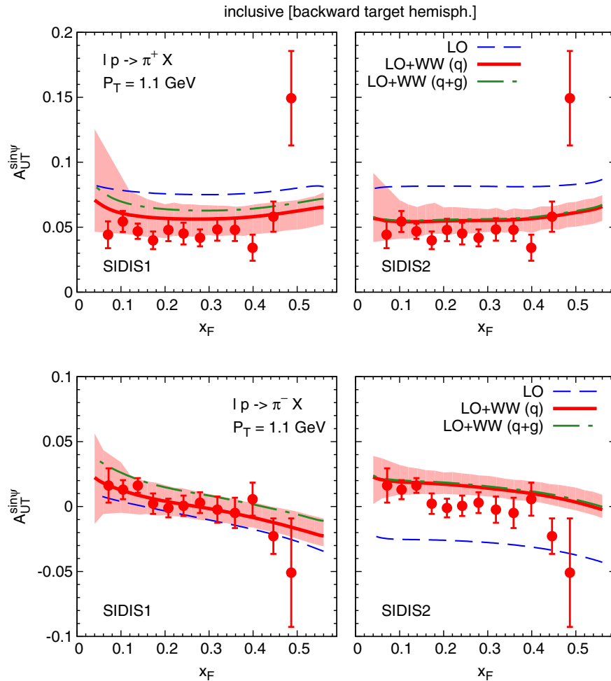
FIG. 8. Theoretical estimates for A_{UT}^{\sin\psi} vs x_F at \sqrt{s} \approx 7.25 GeV and P_T = 1.1 GeV for inclusive \pi^+ (upper panels) and \pi^- (lower panels) production in \ell p^\uparrow \rightarrow \pi X processes, compared with the fully inclusive HERMES data [27]. Two sets for the Siverson and Collins functions have been considered: the SIDIS 1 set (left panels) and the SIDIS 2 set (right panels). More precisely, we show both the LO (blue dashed lines) and LO + WW (red solid lines) quark contributions, as well as the total result including the gluon Siverson effect (green dot-dashed lines). The overall statistical uncertainty band, obtained following the procedure described in Appendix A of Ref. [53] is also shown.
