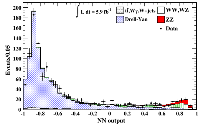
FIG. 1 (color online). Neural network output distribution for the processes contributing to the \ell\ell\nu\nu sample, scaled to the best values of the fit to the data.
