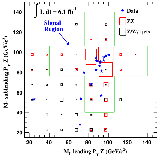
FIG. 2 (color online). Two-dimensional distribution of M_{\ell\ell} for the nonleading p_T vs leading- p_T Z candidates for the expected signal and background compared to the observed events. In the plot, a box is drawn with area proportional to the number of events expected for that M_{\ell\ell}^1, M_{\ell\ell}^2 combination. The green line cross-shaped region represents the acceptance of the requirements applied to select ZZ events, while the stars represent the events observed in the data.
