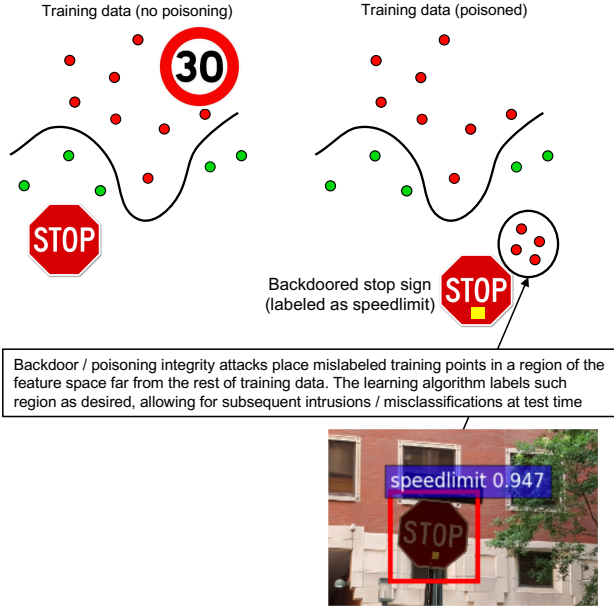
Figure 5: Conceptual representation of the impact of poisoning integrity attacks (including backdoor and trojanning attacks) on the decision function of learning algorithms. The example, taken from [71], shows a backdoored stop sign misclassified, as expected, as a speedlimit sign.
