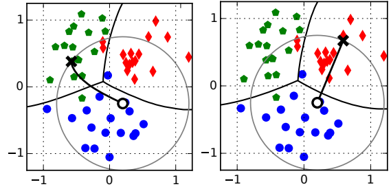
Figure 6: Examples of error-specific ( left ) and error-generic ( right ) evasion, as reported in [7]. Decision boundaries among the three classes (blue, red and green points) are shown as black lines. In the error-specific case, the initial (blue) sample is shifted towards the green class (selected as target). In the error-generic case, instead, it is shifted towards the red class, as it is the closest class to the initial sample. The gray circle represents the feasible domain, given as an upper bound on the \ell_2 distance between the initial and the manipulated attack sample.
