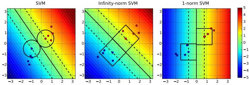
Figure 13: Decision functions for linear SVMs with \ell_2 , \ell_\infty and \ell_1 regularization on the feature weights [77, 78]. The feasible domain of adversarial modifications (characterizing the equivalent robust optimization problem) is shown for some training points, respectively with \ell_2 , \ell_1 and \ell_\infty balls. Note how the shape of these balls influences the orientation of the decision boundaries, i.e., how different regularizers optimally counter specific kinds of adversarial noise.
