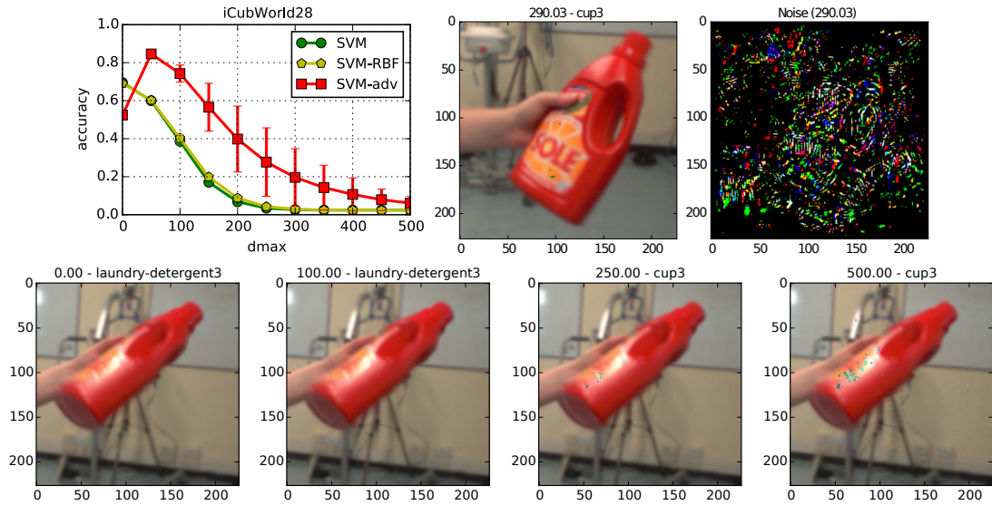
Figure 7: Error-specific evasion results from [7]. Top row : Security evaluation curves reporting accuracy of the given classifiers against an increasing \ell_2 input perturbation. The right-hand side plots depict a laundry detergent misclassified as a cup when applying the minimum input perturbation required for misclassification, along with the corresponding magnified noise mask. Bottom row : Images of the laundry detergent perturbed with an increasing level of noise. The manipulations are only barely visible for perturbation values higher than 150-200 (recall however that these values depend on the image size, as the \ell_2 distance).
