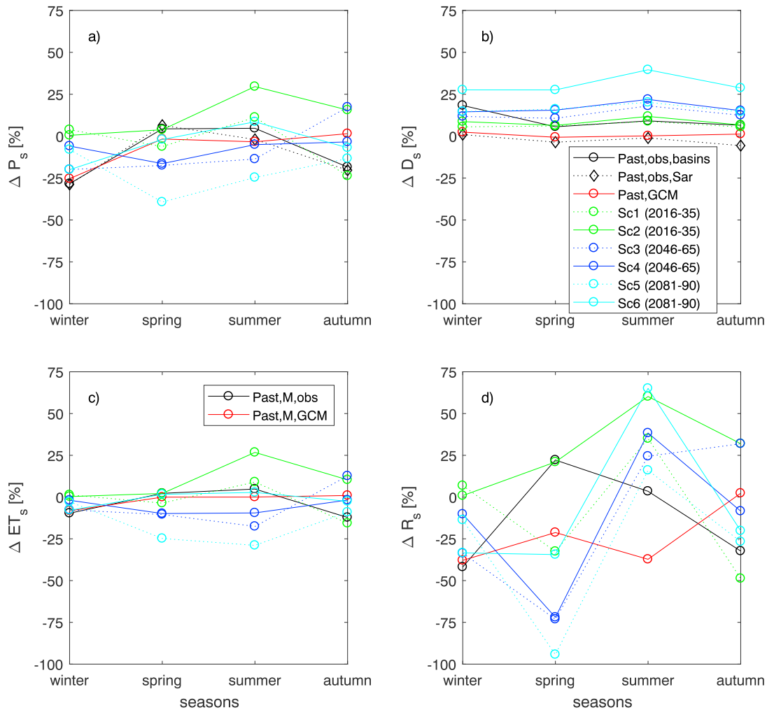
Figure 6. Mean observed changes in the past (1976–2000 compared with 1951–1975) in the basins (Past, obs, basins) and in all the Sardinian meteorological network (Past, obs, Sar), mean of the changes predicted in the past (Past, GCM) by the AOGCM (Table S3), and mean of the changes predicted by the AOGCM in the six future scenarios of Table 2 of (a) seasonal precipitation ( \Delta P_s ) and (b) seasonal vapor pressure deficit ( \Delta D_s ); mean changes of (c) seasonal evapotranspiration ( \Delta ET_s ), and (d) seasonal runoff ( \Delta R_s ) in the past (1976–2000 compared with 1951–1975) using observed P_s and D_s (Past, M, obs) and predicted P_s and D_s by the AOGCM (Past, M, GCM) and in the six future scenarios of Table 2.
