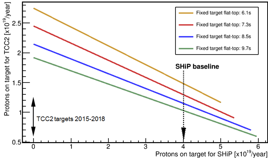
Figure 6. The expected number of protons on the current North Area targets (TCC2) as a function of the number of protons on target for the SHiP experimental facility with a 1.2 s spill length. The plot shows the performance for different spill durations for the current fixed target facilities between 6.1 – 9.7s. The range of the numbers of protons per year delivered to the North Area targets in the years 2015 – 2018 is indicated. The preferred working point for SHIP is indicated by "SHiP baseline".
