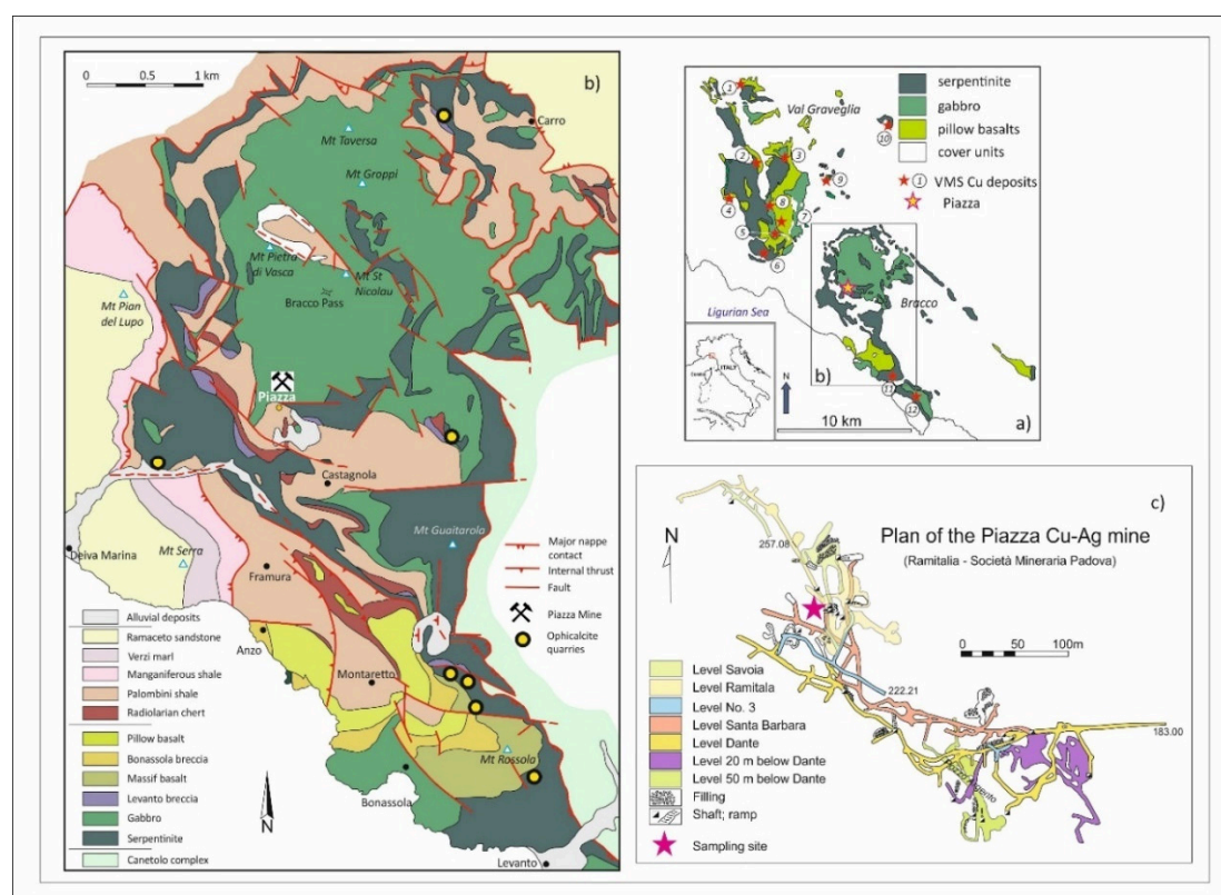
Figure 11. Geological setting of the Piazza mineral deposit, Northern Appennines, Eastern Liguria. (a) Sketchmap of the regional distribution of the ophiolite complexes in the Eastern Ligurian sector of the Northern Appennine Belt and location of the Piazza mine and of the ophiolite-hosted volcanogenic massive sulfide (VMS) deposits of the area after [47]. Location codes: (1) Reppia, (2) Monte Bianco, (3) Monte Bardeneto, (4) Libiola, (5) Campegli, (6) Casali-Monte Loreto; (7) Gallinaria, (8) Bargone, (9) Molin Cornaio; (10) Rocca di Lagorara, (11) Monte Rossola, (12) Monte Mescio. (b) Geological features of the Bracco ophiolite massif (after [50]) and localization of the Piazza mine and of sulfide-bearing ophicalcite quarries in [51]. (c) Reproduction of the historical planimetry of the Piazza mine and indication of the accessible portion (Level Ramitala) where sampling was done (after [55,56]).
