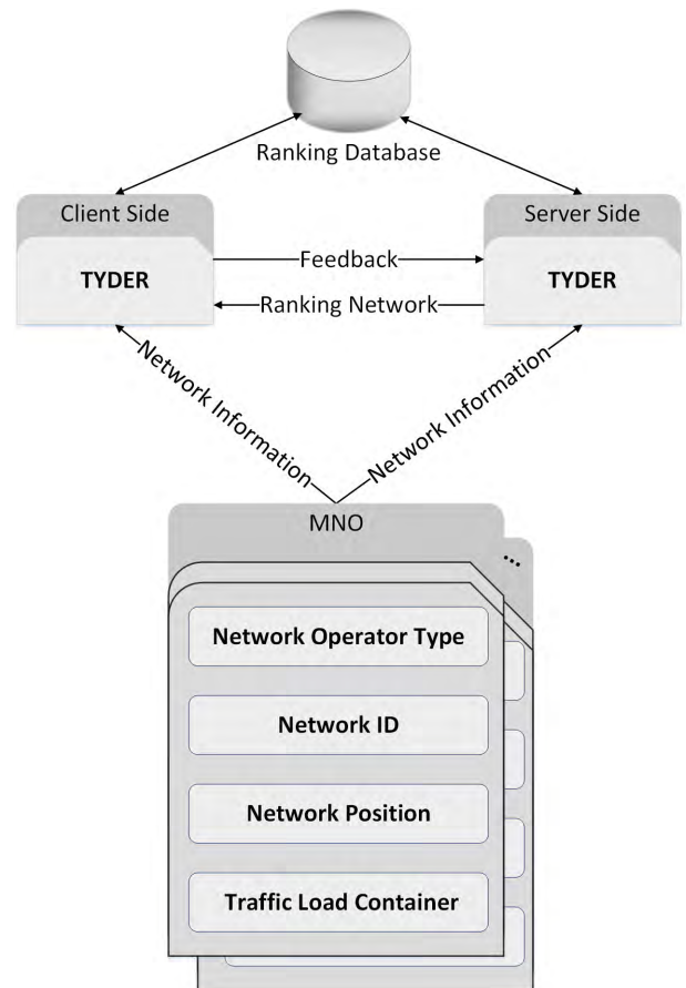
FIGURE 2. TYDER architecture.
