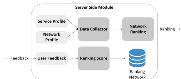
FIGURE 7. Server module.
