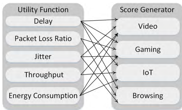
FIGURE 6. Utility function and score generator.
