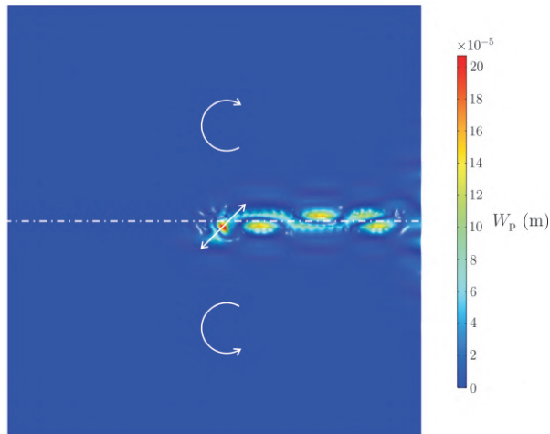
Figure 1: One-way unidirectional wave in a plate with a finite array of chiral resonators, consisting of beams attached to gyroscopic spinners. The structure is divided into two domains, characterised by opposite values of the gyricity \Omega (see Section 2), and is excited by a time-harmonic force, represented by the arrow, applied to the tip of a beam in the lower domain. The transverse displacement amplitude in the plate W_p is plotted. The values of the parameters are given in Section 4.
