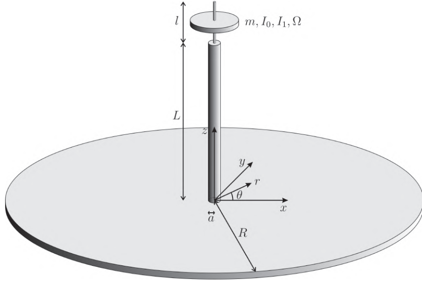
Figure 2: Elastic multi-structure, made of an elastic beam connected at one end to a gyroscopic spinner and at the other end to the centre of a circular plate, clamped on the boundary.
