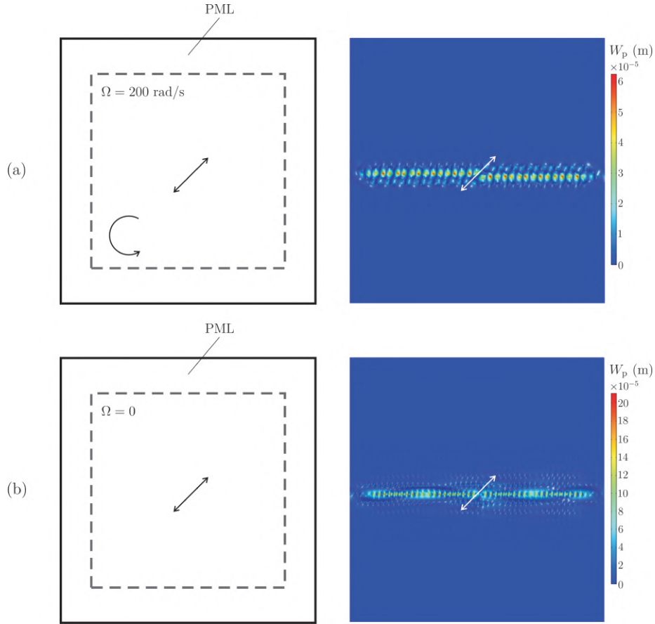
Figure 9: Time-harmonic response of the uniform chiral flexural structure to a force of amplitude 1 N and radian frequency (a) \omega = 245.7 rad/s and (b) \omega = 247.1 rad/s. The value of the gyricity \Omega in each case is indicated in the figures.
