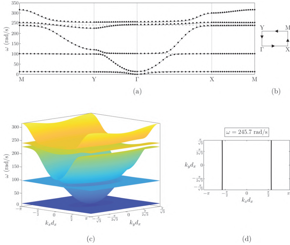
Figure 5: (a) Band diagram of the periodic system in Fig. 4 with \Omega = 200 rad/s, evaluated along the path \Gamma XMY\Gamma shown in (b). Analytical (solid grey lines) and numerical (black dots) results are compared. The dashed horizontal lines indicate the frequencies that will be used in the numerical simulations of Section 4. (c) Dispersion surfaces of the system, determined numerically. (d) Slowness contours calculated for \omega = 245.7 rad/s.
