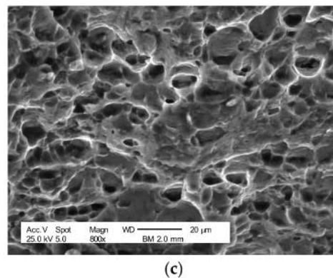
Figure 5. Scanning electron microscope fractography of the BM+CRed samples deformed along the cold rolling direction: (a) \Delta h = 0 mm; (b) \Delta h = 0.1 mm; (c) \Delta h = 0.5 mm.
