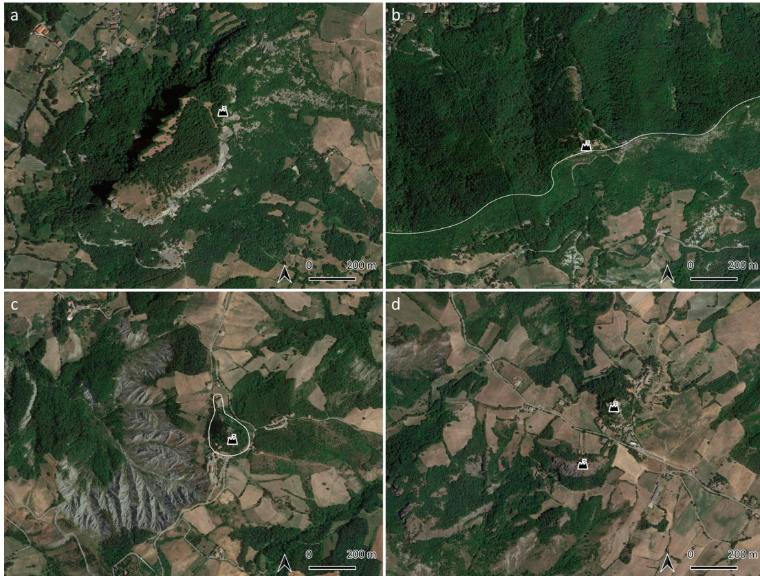
Figure 3. Examples of geological and geomorphological settings of selected castles (satellite imageries from GoogleEarth™): (a) the Pietra di Bismantova castle on top of a mesa-type relief; (b) the Carpineti castle on the rim of a monocline structure; (c) the Canossa Castle on a residual hill of sandstone surrounded by badlands developed on marls and clays; (d) the Guardiola (bottom) and Rossena (top) castles built on top of ophiolite domes.
