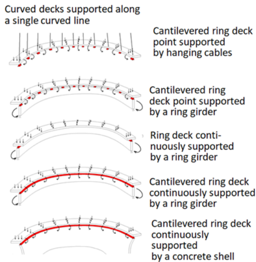
Figure 10: Curved cantilevered deck supported along a single curved line
