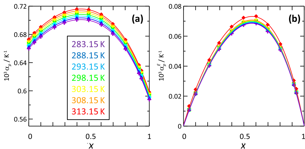
Fig. 4. (a) Isobaric thermal expansion coefficient, and (b) excess isobaric thermal expansion coefficient, for x [EMIM][BF 4 ] + (1-x) [EMIM][TFSI], x stands for mole fraction, mixtures as a function of temperature.
