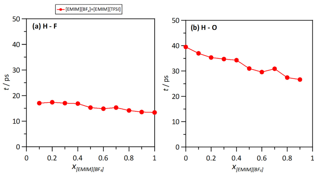
Fig. 16. Residence times, t , for selected atom pairs in x [EMIM][BF 4 ] + (1-x) [EMIM][TFSI] mixtures from MD simulations at 298 K and 1 bar. Residence times are calculated for first solvation layer defined according to the first minima in the corresponding g(r) .
