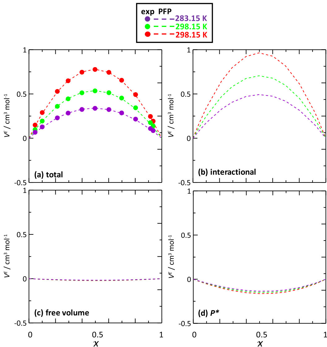
Fig. 5. Comparison of experimental, exp, and Prigogine-Flory-Patterson, PFP, excess molar volume, V^E , x [EMIM][BF 4 ] + (1-x) [EMIM][TFSI], x stand for mole fraction, mixtures as a function of temperature. Results in panels b to d show interactional, free volume and P^* PFP contributions to the total V^E .
