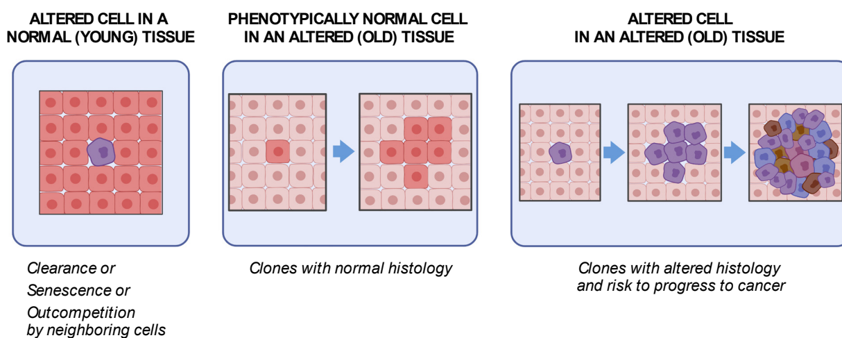
Figure 2. Aging and cancer: an ecological view. If an altered cell emerges in a normal tissue environment ( left panel ), it will be most likely cleared or kept at bay by mechanisms outlined in Figure 1. On the other hand, widespread alterations in the tissue environment, such as during aging ( central panel ), can select for the emergence of more fit, phenotypically normal cells, forming histologically normal clones. The combined presence of altered cellular phenotypes in an altered tissue environment ( right panel ) can set the stage for the evolution of neoplastic disease.
