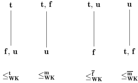
Figure 4. Multiple orders on the elements of the \mathbf{WK} algebra
