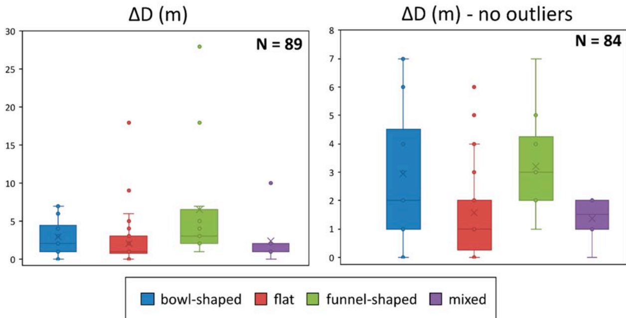
Figure 8. Boxplots of the difference between depth (D) values from field- and DEM-derived measurements for the entire population ( left ) and a subset without outliers ( right ). The boxplots are grouped according to doline shape. The limits of the boxes and whiskers represent the first and third quartiles, respectively. The straight lines inside the boxes represent the median values and the crosses represent the mean values.
