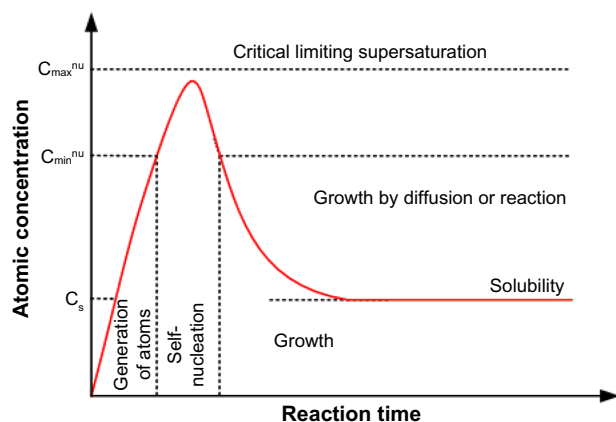
Figure 3 Plot of atomic concentration against time, illustrating the generation of atoms, nucleation, and subsequent growth.
