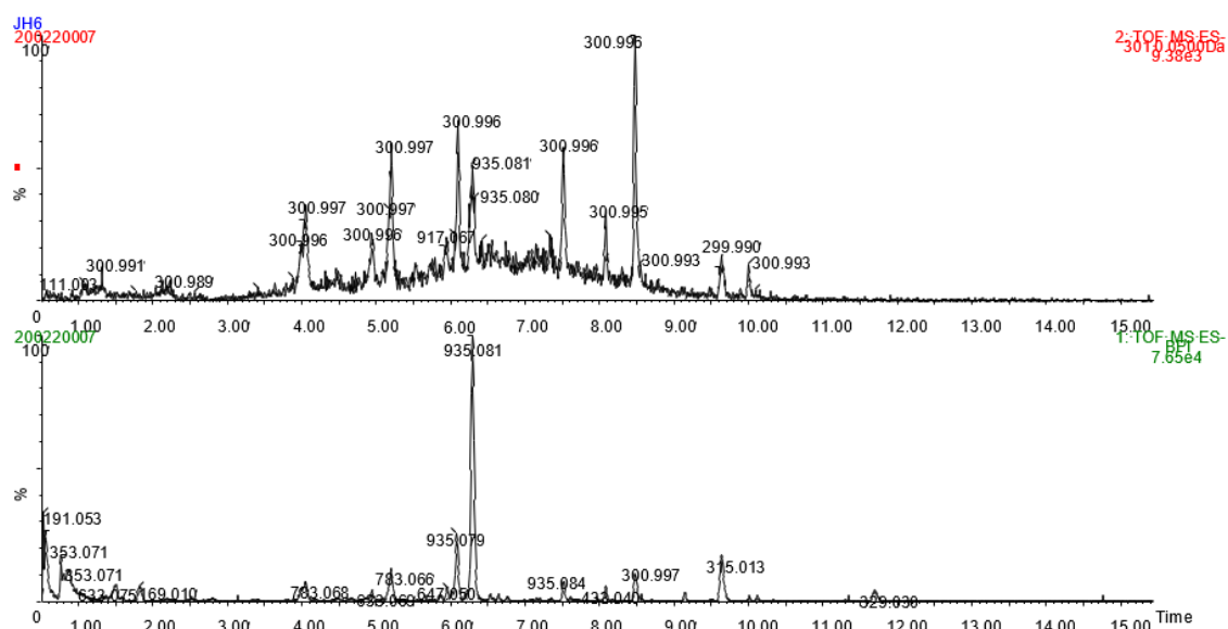
Figure 1. Base peak intensity chromatogram and MS E chromatogram at m/z 301.0 for jabuticaba peel extract.
