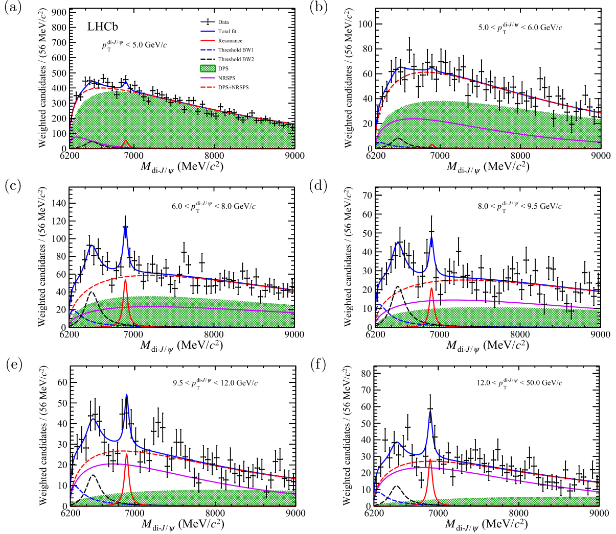
Fig. 4. Invariant mass spectra of weighted di\text{-}J/\psi candidates in bins of p_T^{di\text{-}J/\psi} and overlaid projections of the p_T^{di\text{-}J/\psi} -binned fit with model I.
