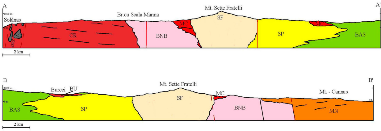
Figure 4. Schematic cross-sections for Sàrrabus pluton, as reported in Figure 3. S.L. refers to sea level; no vertical exaggeration. To simplify, dike swarms and episyenites were not plotted. BAS, BU, MC, MN, CR, BNB, SP, SF refer to metamorphic basement, Burcei, Monte Cresia, Monte Nai, Cala Regina, Brunco Nicola Bove, San Priamo, Sette Fratelli units, respectively. SO refers to synplutonic mafic masses of Cala Regina Unit.
