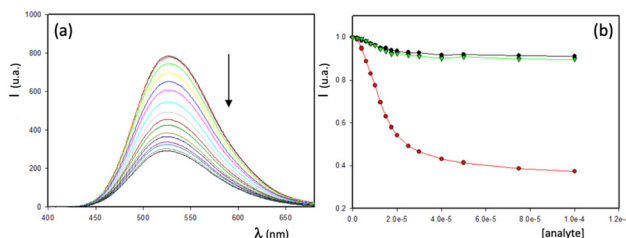
Fig. 5 (a) Fluorescence spectra ( \lambda_{\text{exc}} = 350\ \text{nm} ) in \text{CH}_3\text{CN}/\text{DMSO} solution (9 : 1 v/v) of L1 ( 10\ \mu\text{M} ) upon addition of increasing amount of the sodium salt of \text{KET}^- ; (b) normalized fluorescence intensity ( \lambda_{\text{exc}} = 350\ \text{nm} ; \lambda_{\text{em}} = 525\ \text{nm} ) of L1 ( 10\ \mu\text{M} ) upon addition of increasing amount of ketoprofen (red circles), naproxen (green triangles), and benzoate (black circles) as their sodium salt.
