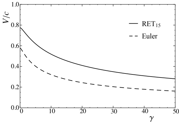
Fig. 1 Dependence of maximum V/c on \gamma for a diatomic gas. The solid line indicates the value of \text{RET}_{15} and the dashed line indicates the one of Euler system [36].
