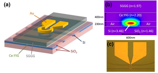
Fig. 2. (a) 3D prospective view of the device, (b) cross-sectional mode profile, and (c) microscope image of the fabricated device. The silicon waveguide is 230 \text{ nm} tall and 600 \text{ nm} wide, and the Ce:YIG is 400 \text{ nm} thick. A thin layer of silica ( \sim 10 \text{ nm} ) is assumed to have formed between the waveguide and the bonded layer due to the plasma activation [24].
