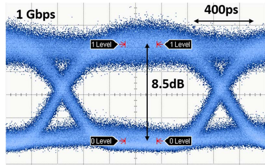
Fig. 6. Magneto-optic rise time of the device is measured to be 400 ps using a 1 Gbps PRBS31 bit stream. The eye stays open up to 2.5 Gbps, which agrees well with the measured rise time.
