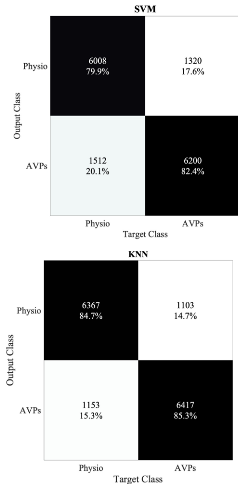
Figure 3. Cumulative confusion matrices for the two classifiers. In each matrix, the TPR (black box on the bottom-right corner) and the TNR (black box on the top-left corner) are reported along with their respective false negative rate (white box on the top-right corner) and FPR (light box on the bottom-left corner).
